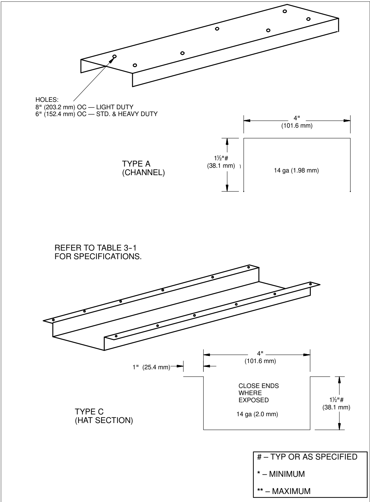
FIGURE 3-4 UNDERBRACING DETAILS
