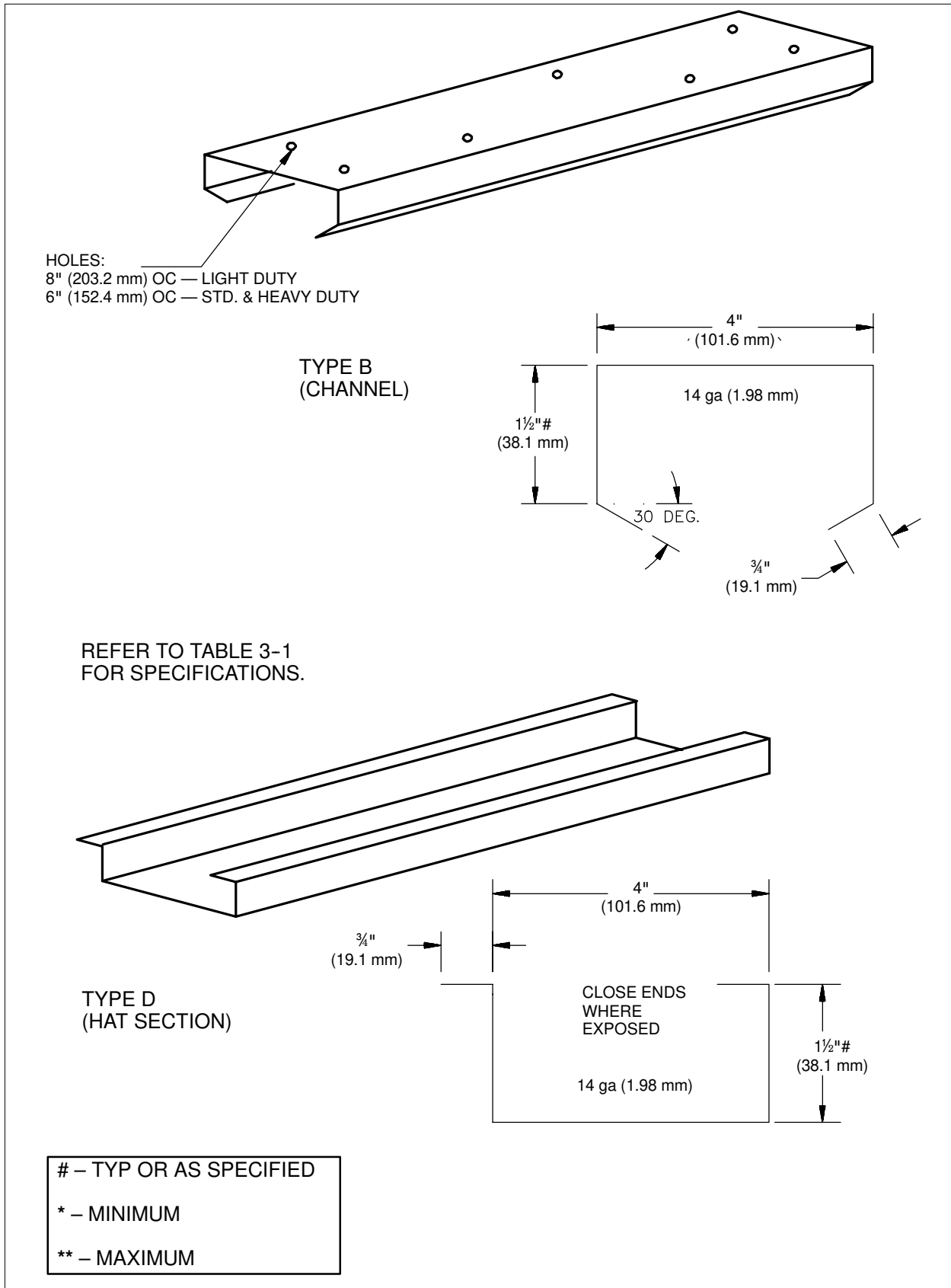
FIGURE 3-5 UNDERBRACING DETAILS
