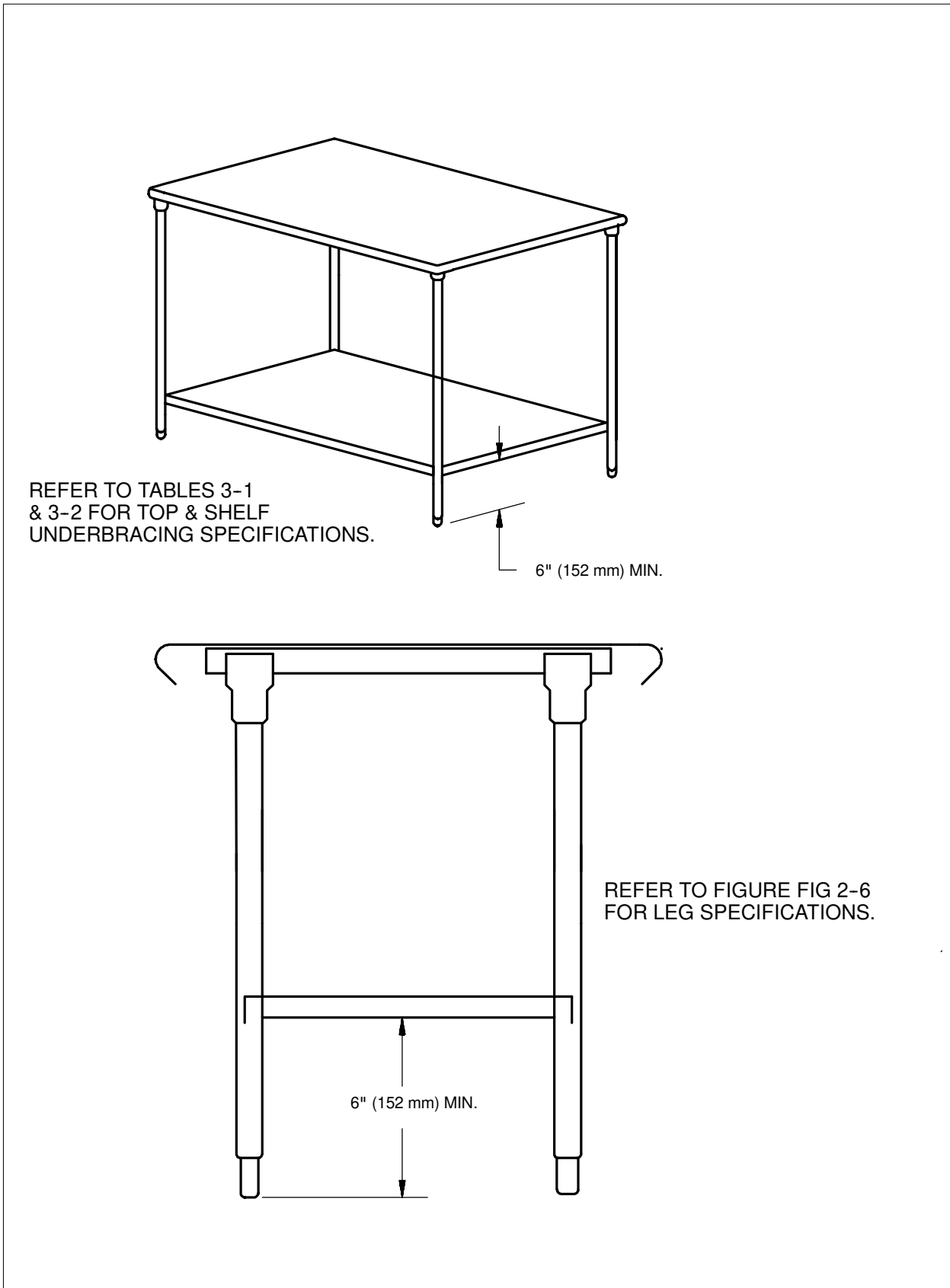
FIGURE 3-1 WORK TABLE
